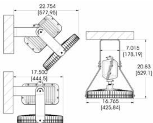
HLXW3-SS - Swivel Bracket
